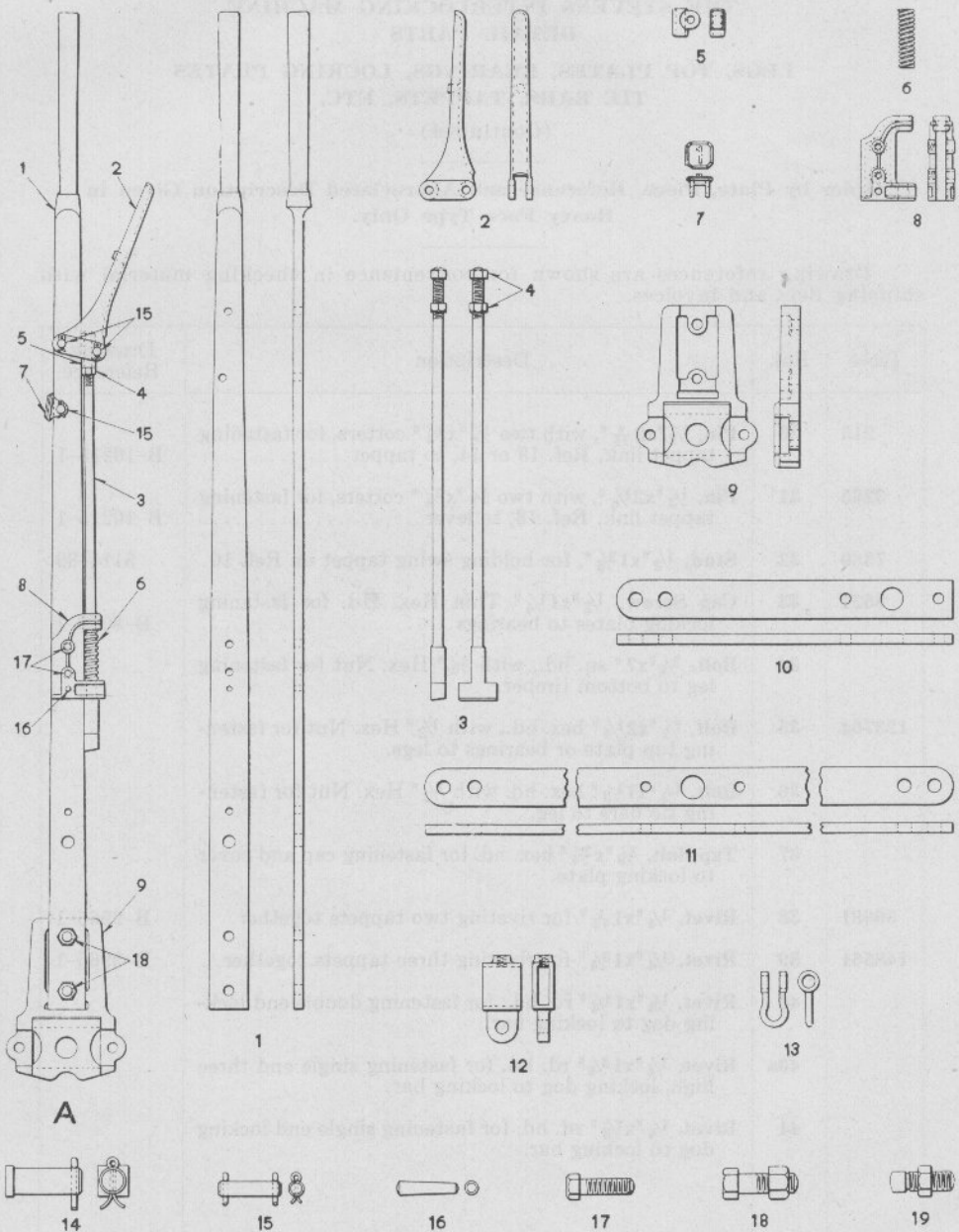
LEVERS AND DETAILS FOR STEVENS INTERLOCKING MACHINE
